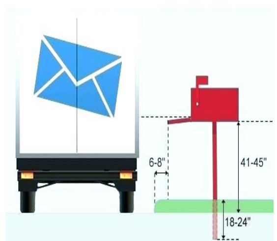
Standard Dimensions for a Mailbox
